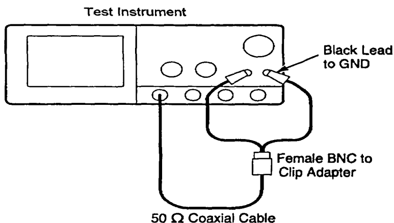
Figure 8. Equipment setup.
